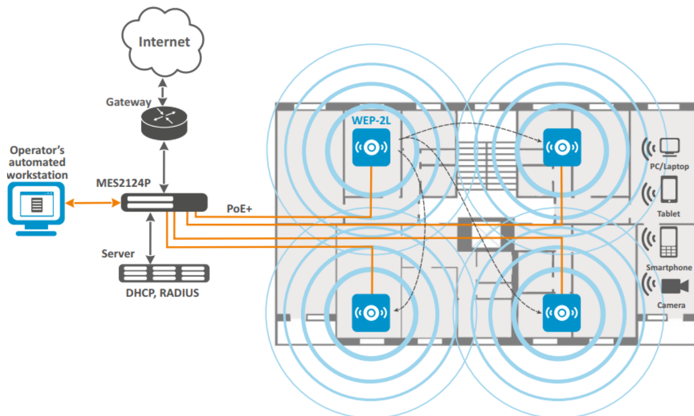
Figure 1 – WEP-2L application scheme
